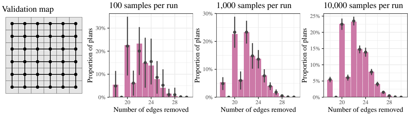
Figure 4: The 6-by-6 map used in validation (left). The remaining panels compare the distribution of the number of removed edges in the enumerated distribution (purple bars) and the sampled distribution (grey) over a number of sample sizes S . The dots are the mean histogram estimate across the 24 independent runs, and represent the algorithm’s bias. The vertical lines are 90% confidence intervals for the histogram estimates, and represent the sampling variability. They are calculated from the standard deviation of the estimates across the runs.
