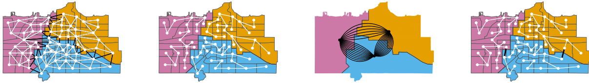
(a) The Erie graph. Edges that cross from one administrative unit to another are colored black. (b) Spanning trees drawn on each administrative unit. (c) The quotient multigraph. Edges connecting boundary units in the original graphs become edges in the multigraph. (d) The final spanning tree. A spanning tree on the quotient multigraph connects the trees on each administrative unit.
