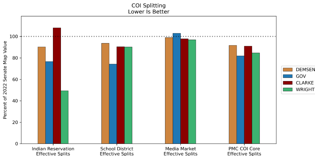
Figure 9. Community-of-Interest Integrity—Senate.
